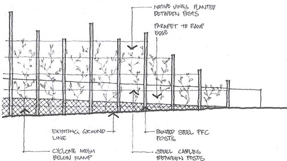
PART ELEVATION NTS
